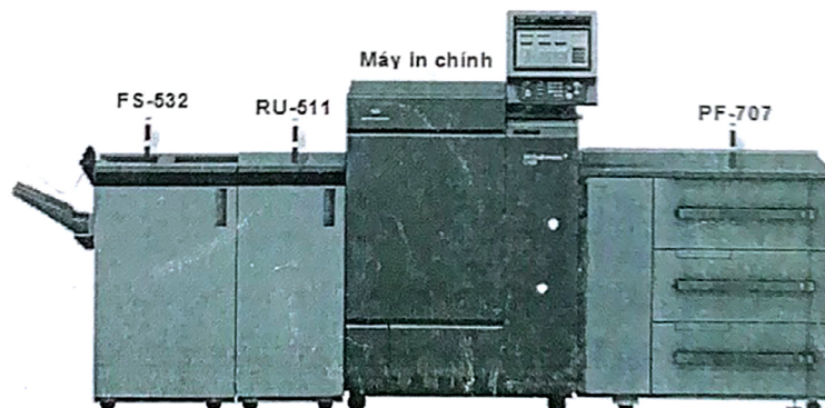
Size ( W x H x D ) = 2,850 x 1,319 x 950 mm
